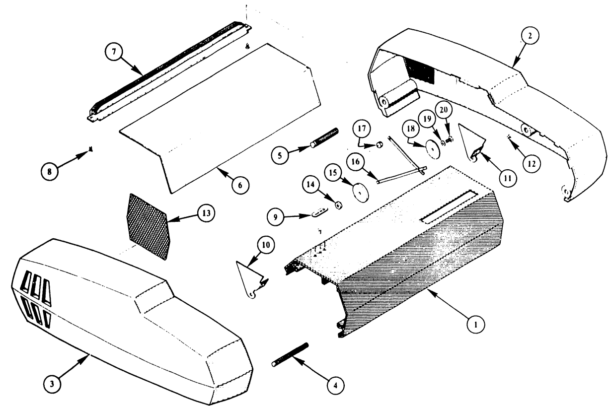
FIGURE 8-1 COVER ASSEMBLY
