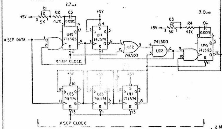
FM DATA SEPARATOR
