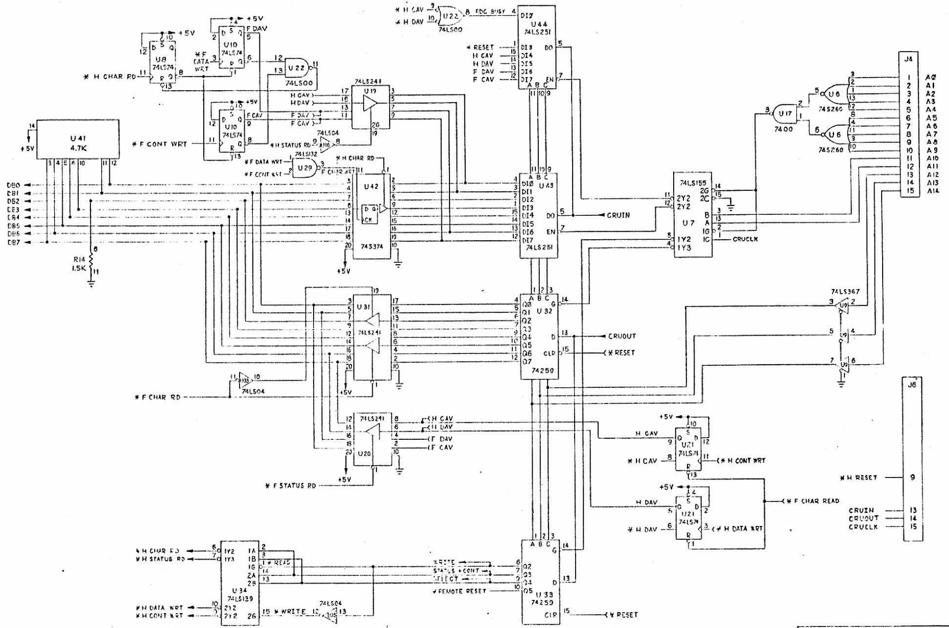
TEC-9900-FDC FLOPPY DISC CONTROLLER J5 EXP. PORT SHEET 2 OF 3
