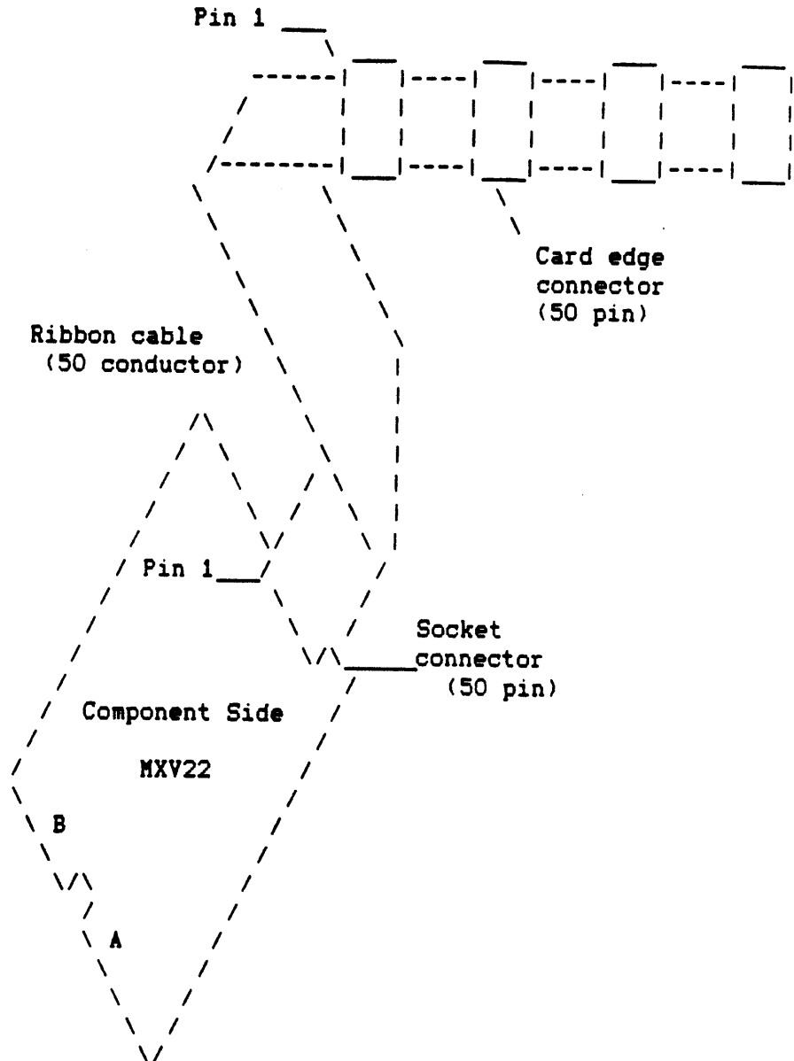
Figure 2-2: Drive/Controller Cabling
