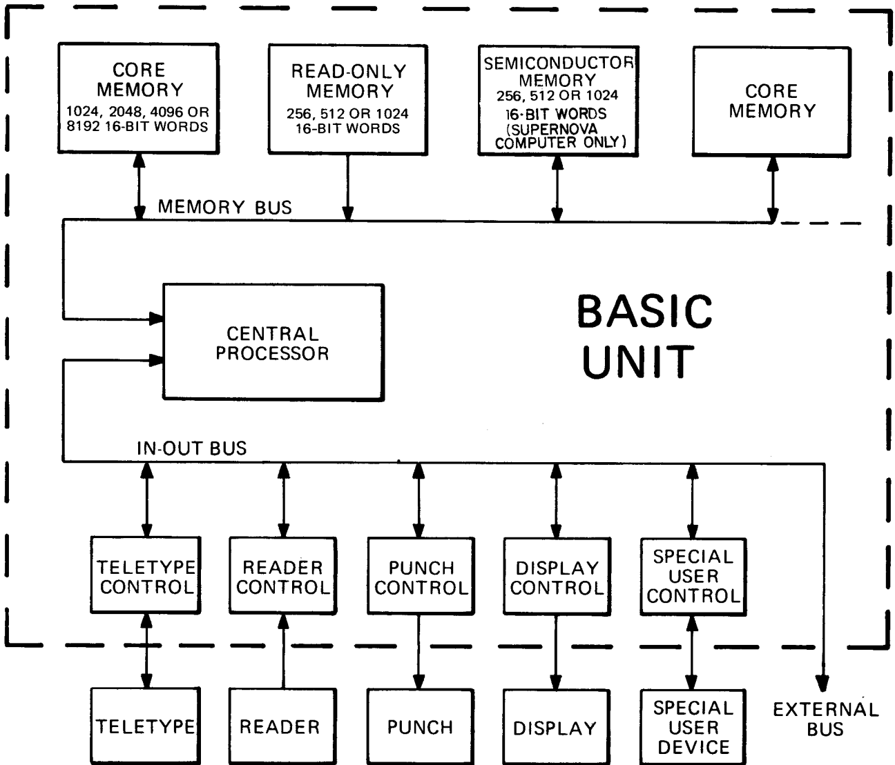
TYPICAL NOVA COMPUTER SYSTEM CONFIGURATION
