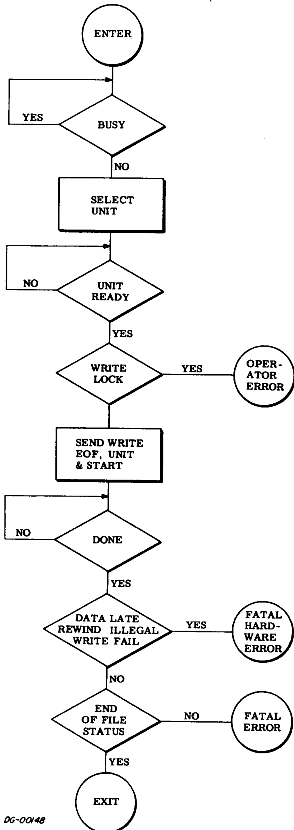
DGC Cassette WRITE END OF FILE Flowchart
