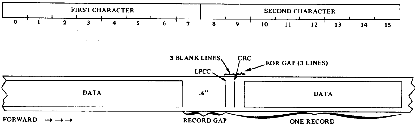
9-TRACK FORMAT
