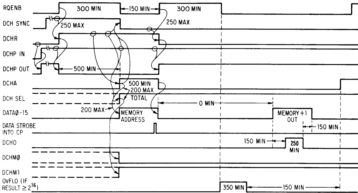
STANDARD DATA CHANNEL CYCLE: INCREMENT MEMORY
