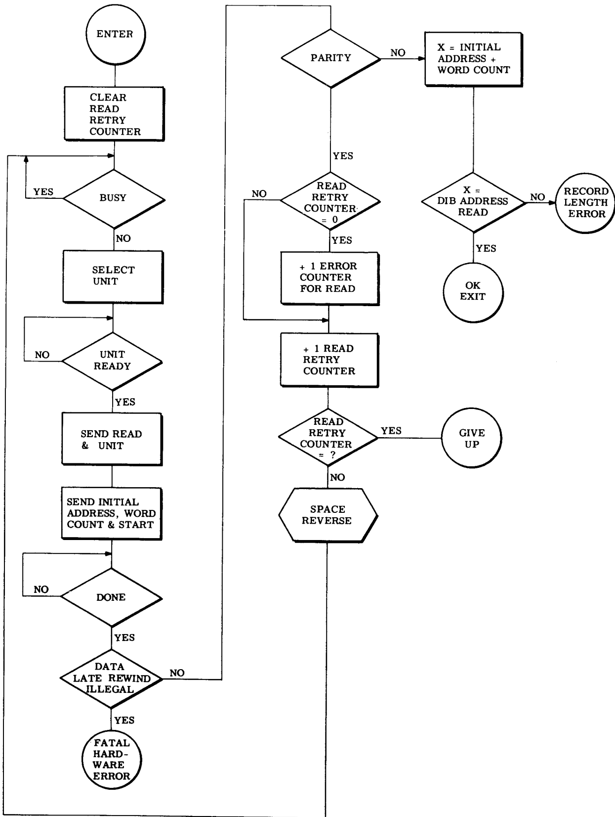
DGC Cassette READ Flowchart
