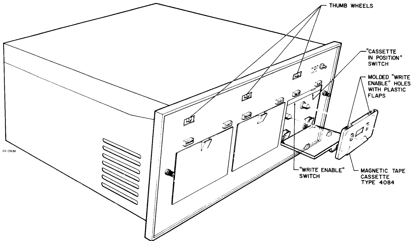
The DGC Cassette Chassis
