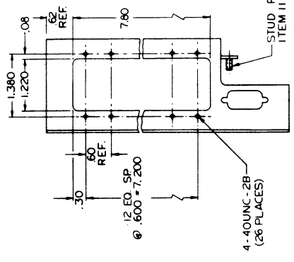
VIEW F-F SCALE: FULL SIZE
