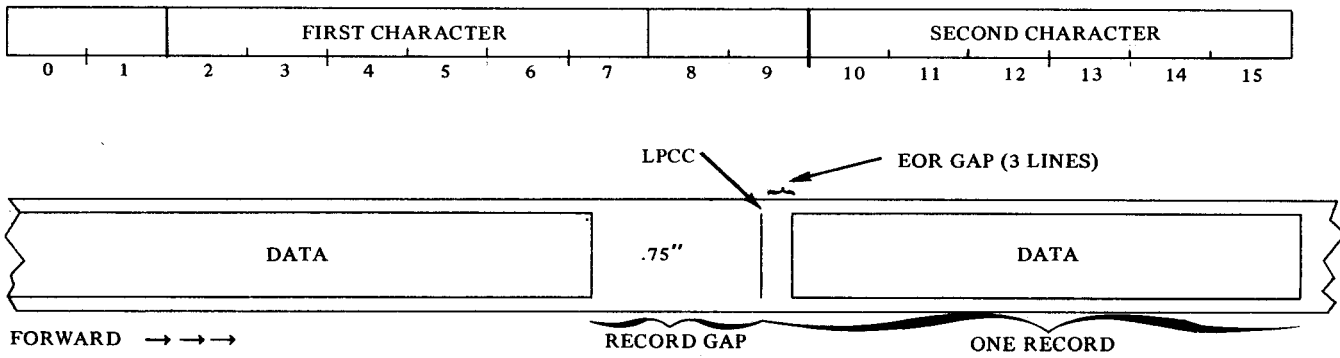
7-TRACK FORMAT
