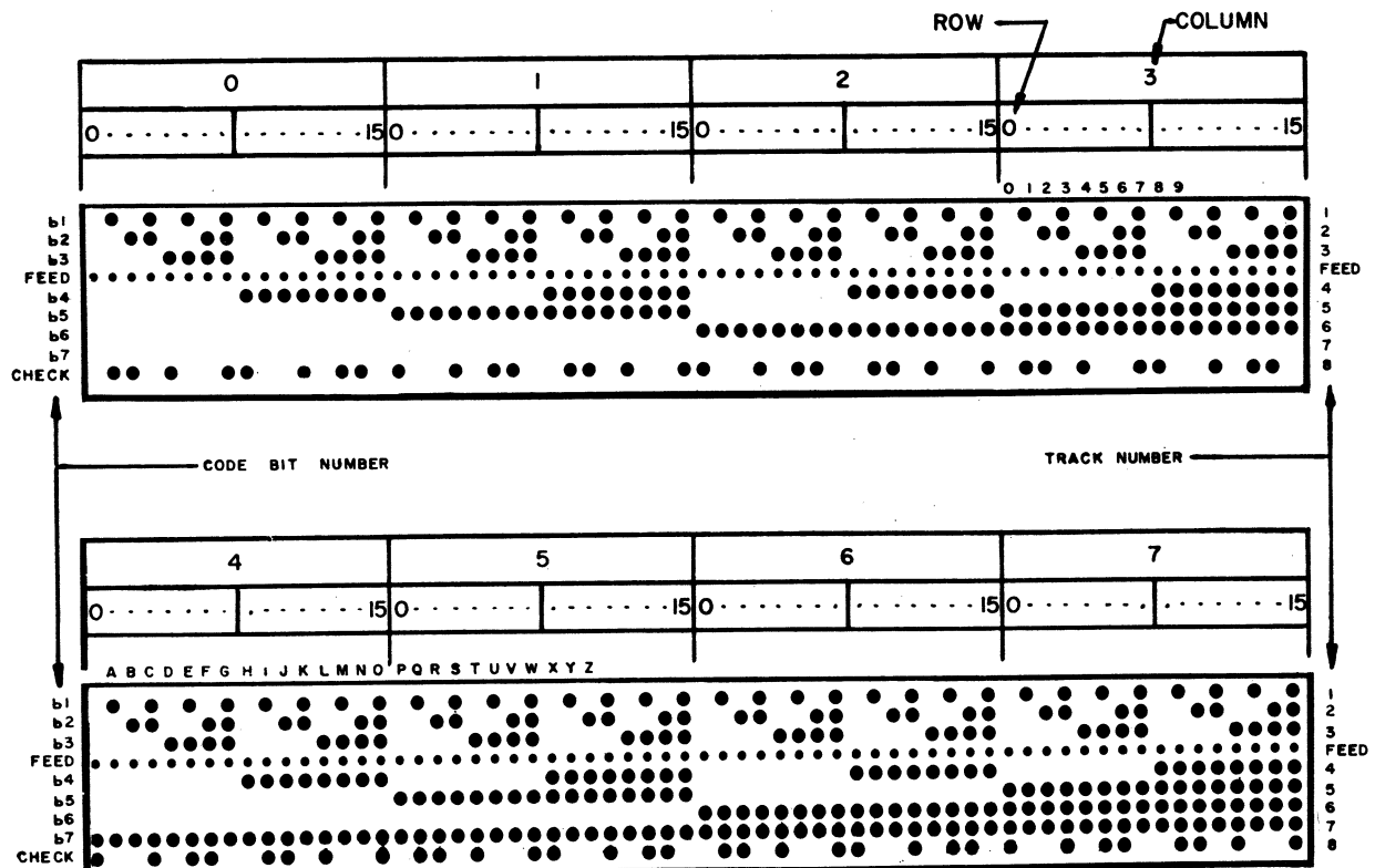
Fig. 1 Perforated Tape Code
