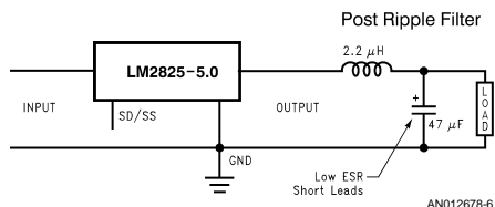
FIGURE 5. Post Ripple Filter
