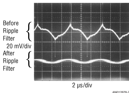
FIGURE 6. Post Ripple Filter Waveform
