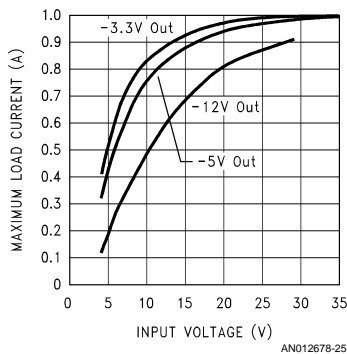
FIGURE 17. Inverting Regulator Typical Load Current
