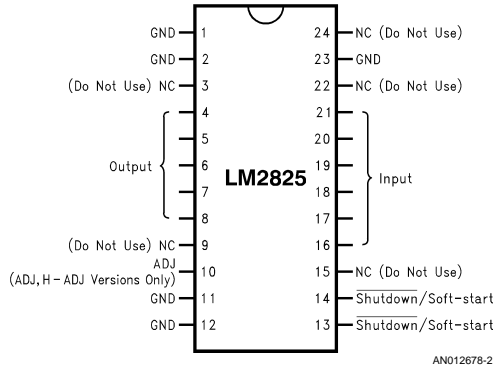
FIGURE 1. Connection Diagram
