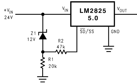
FIGURE 14. Undervoltage Lockout Circuit
