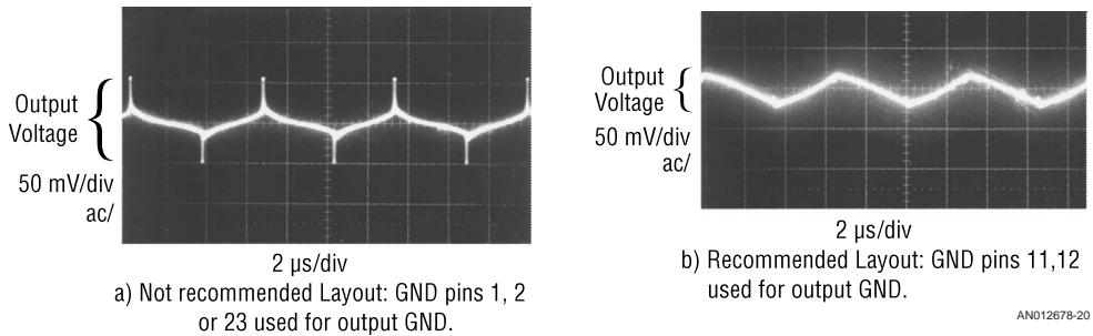
FIGURE 23. Ripple and Spikes at the Output Voltage
