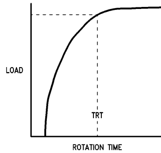
FIGURE 2. Timed Token Protocol
