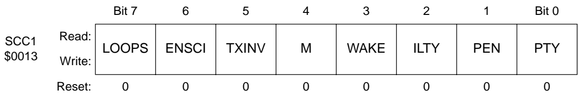
Figure 5. SCI control register 1 (SCC1)
