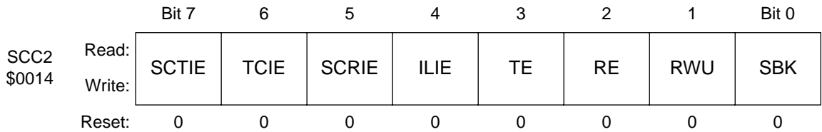
Figure 6. SCI control register 2 (SCC2)
