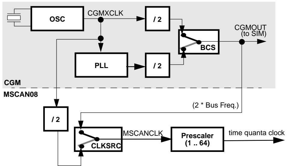
Figure 7. Clocking scheme
