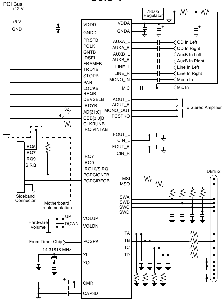
Figure 1 Typical Application
