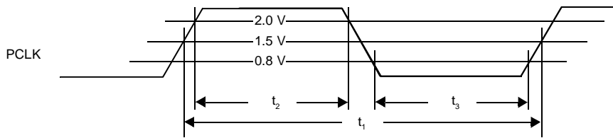
Figure 12 PCLK Timing
