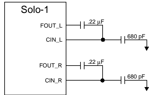
Figure 10 Switched-Capacitor Filter Pin Diagram
