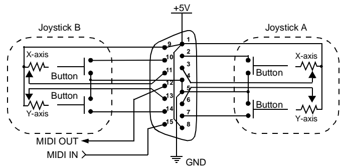
Figure 6 Dual Joystick/MIDI Connector
