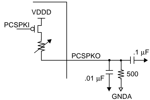
Figure 8 PC Speaker Volume Circuitry
