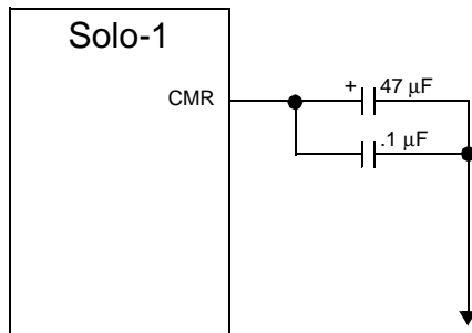
Figure 9 Reference Generator Pin Diagram
