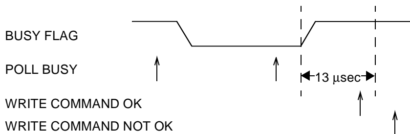
Figure 11 Command Transfer Timing
