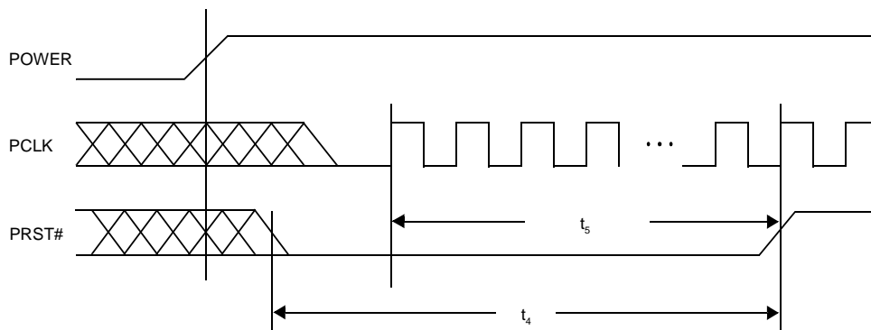
Figure 13 PRST Timing
