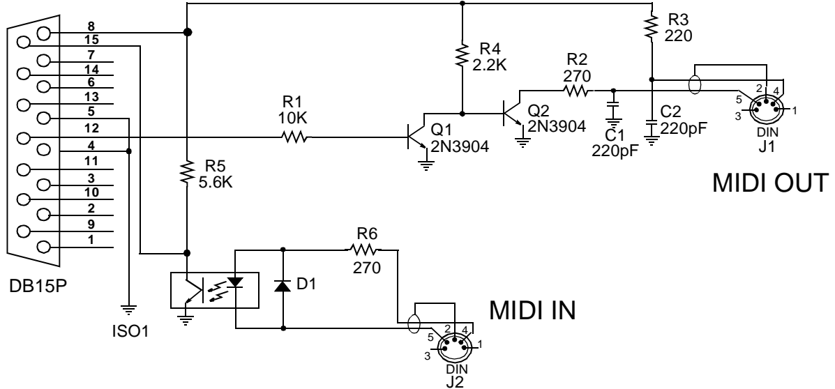
Figure 7 MIDI Serial Interface
