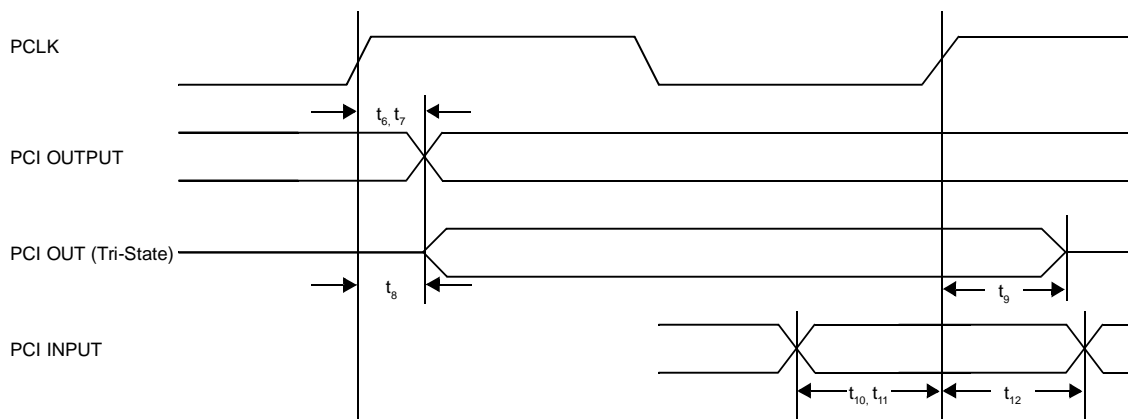
Figure 14 PCI Signal Timing 1
