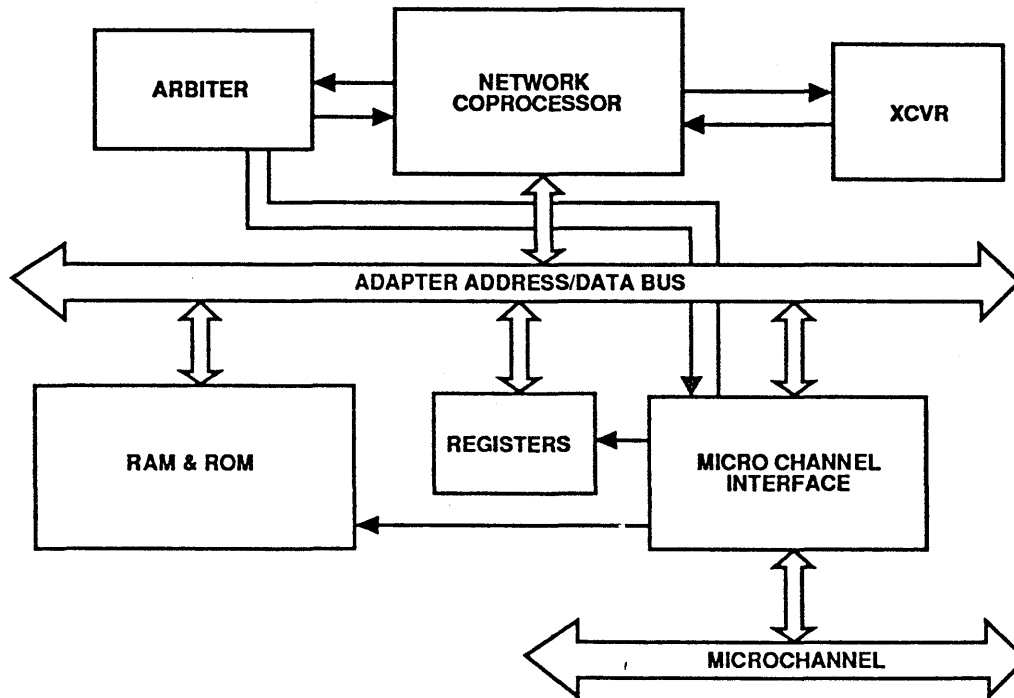
Figure 1-1. EtherLink/MC Adapter Block Diagram
