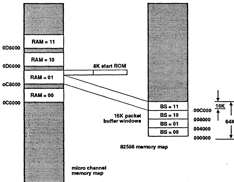
Figure 2-1. Packet Buffer Memory
